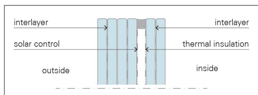
Figure: Sample construction of a bullet resistant insulating
